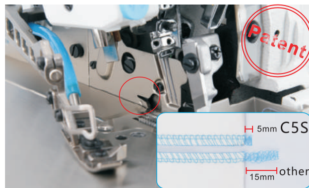
2 Short thread remaining, No need extra trimming
