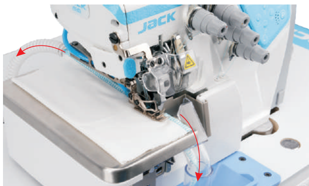
1 Front and Back suction. Clean sewing
