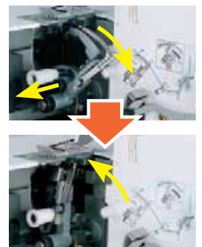
Fast and easy looper threading system
